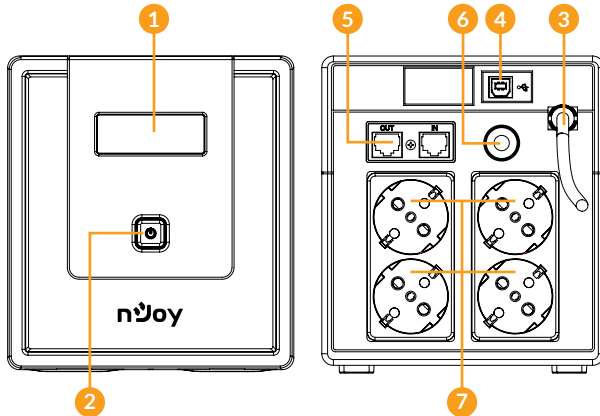
◦ Cadu 1500/2000 - Front view / Back view
