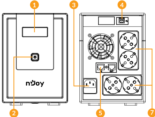
◦ Cadu 1500/2000 - Front view / Back view
