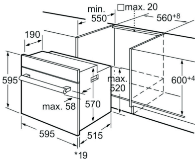
Pic.2 Cabinet Dimensions
