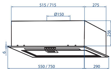
HBI 5664 GLASS 1000 LED Line HBI 7664 GLASS 1000 LED Line
