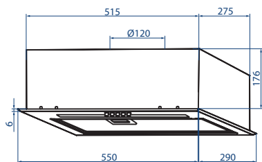
HBI 5264 GLASS 700 LED Line
